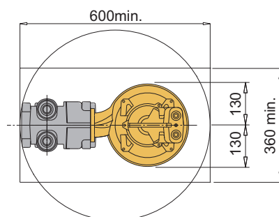
Version with duck foot coupling
