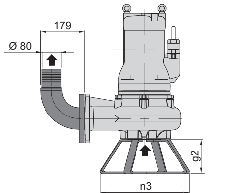
Version with foot and 90° elbow
