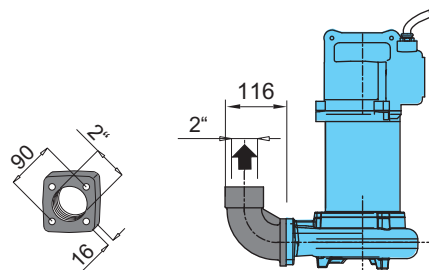
Version with threaded flange and 90° elbow
