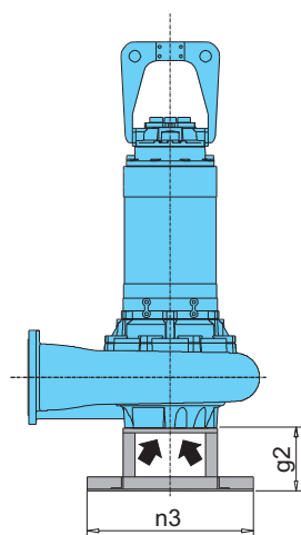
Version with foot
