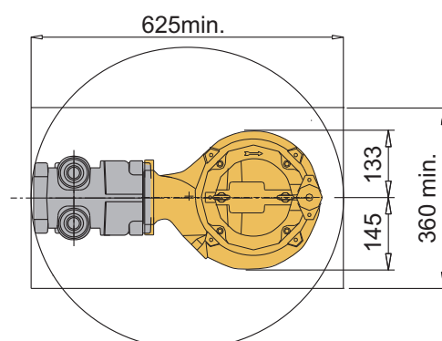
Version with duck foot coupling
